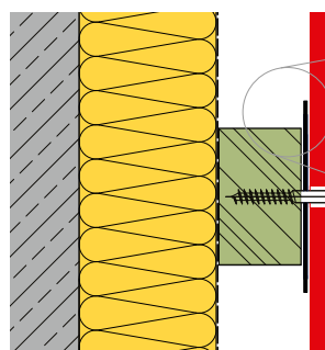
CENTER SUPPORTING LATH A108
